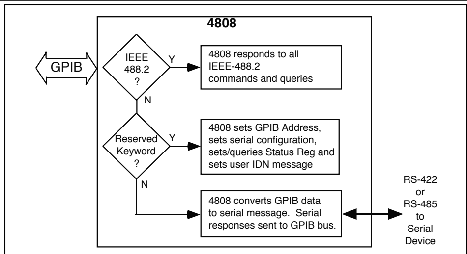
Figure 3 4808 Operation Diagram
