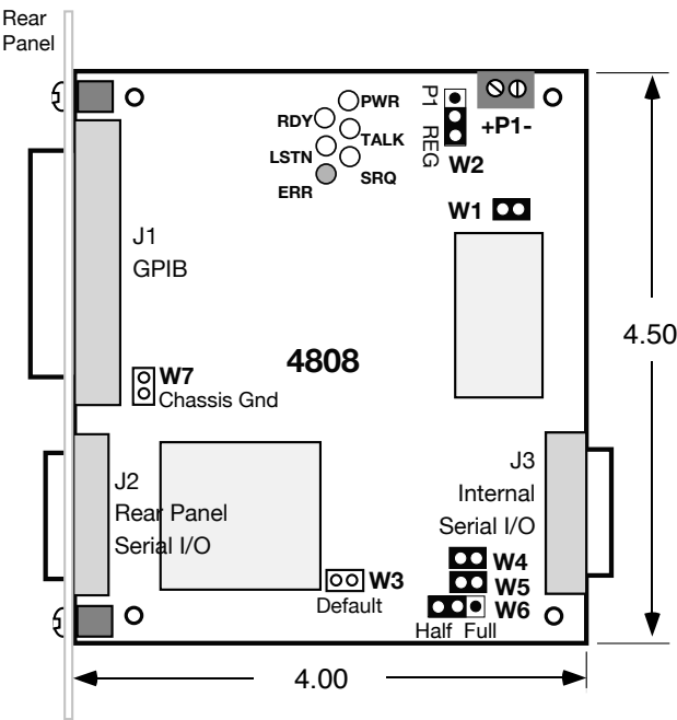
Figure 6 4808 Outline Dimensions
