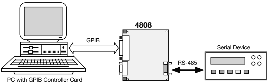
Figure 2(b) 4808 with a Standard Serial Device
