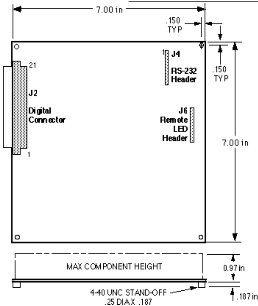
Figure 2 2363 OEM Board Dimensions
